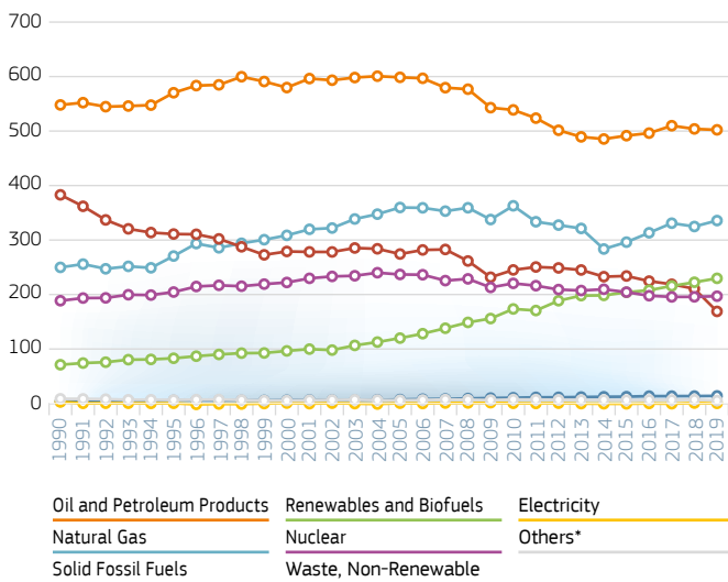
BY FUEL – EU27_2020 – 1990-2019 (Mtoe)
